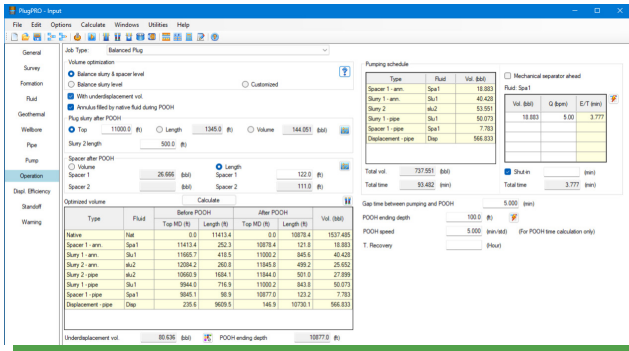
Under-Displacement Volume Calculation
