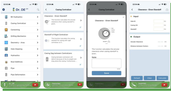
Mobile App
