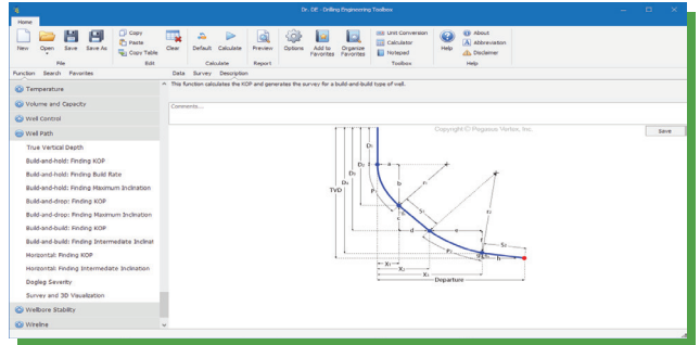
Graph
