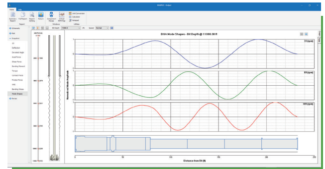
Mode Shape
