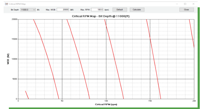
Critical RPM Map
